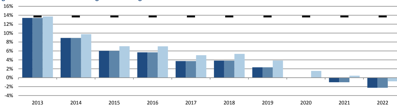
Figure 7: ERCOT Summer Planning Reserve Margins
