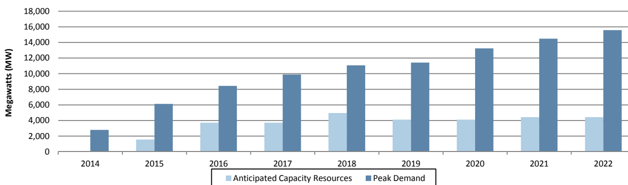
Figure 9: ERCOT – Cumulative Summer Peak Demand Growth Projected to Outpace Supply Resources
